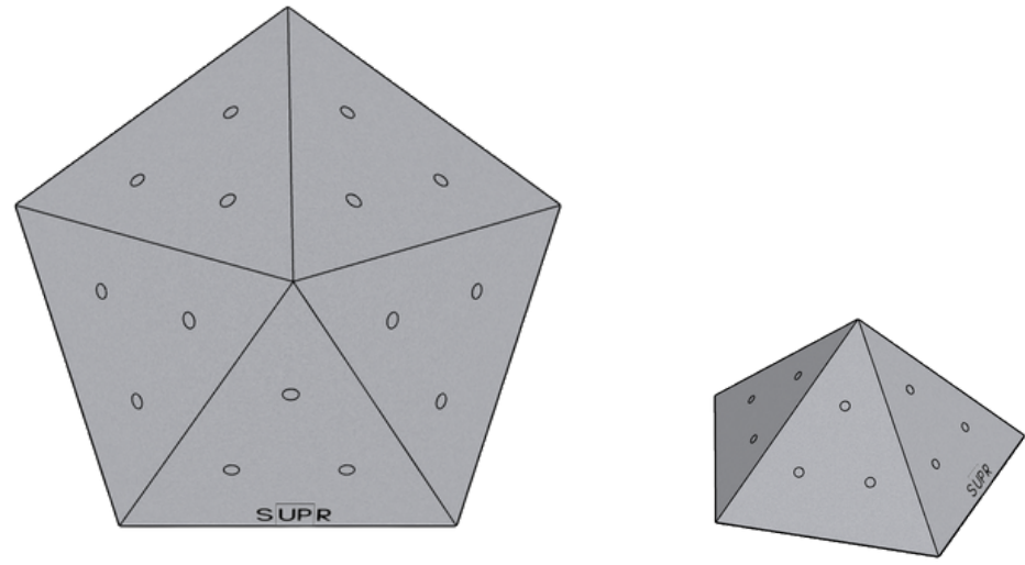
05-02.01 PENTA 2 SIZE S Max Length 45cm Max Height 20cm
